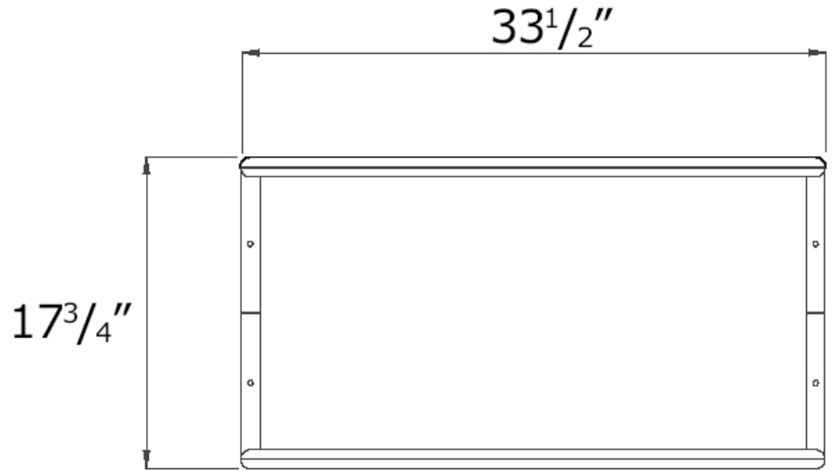
BACK VIEW
