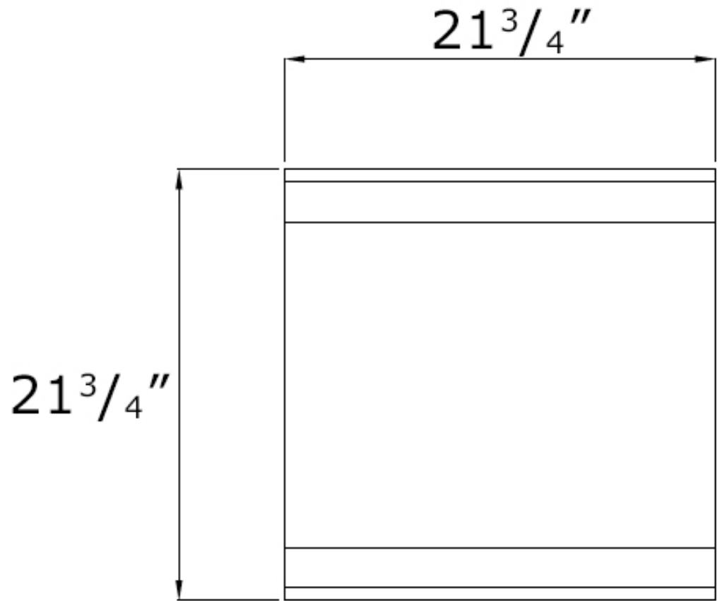
TOP VIEW
