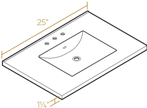
ISOMETRIC
