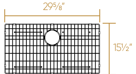
Protective Grid
