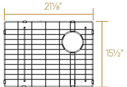
Two Protective Grids
