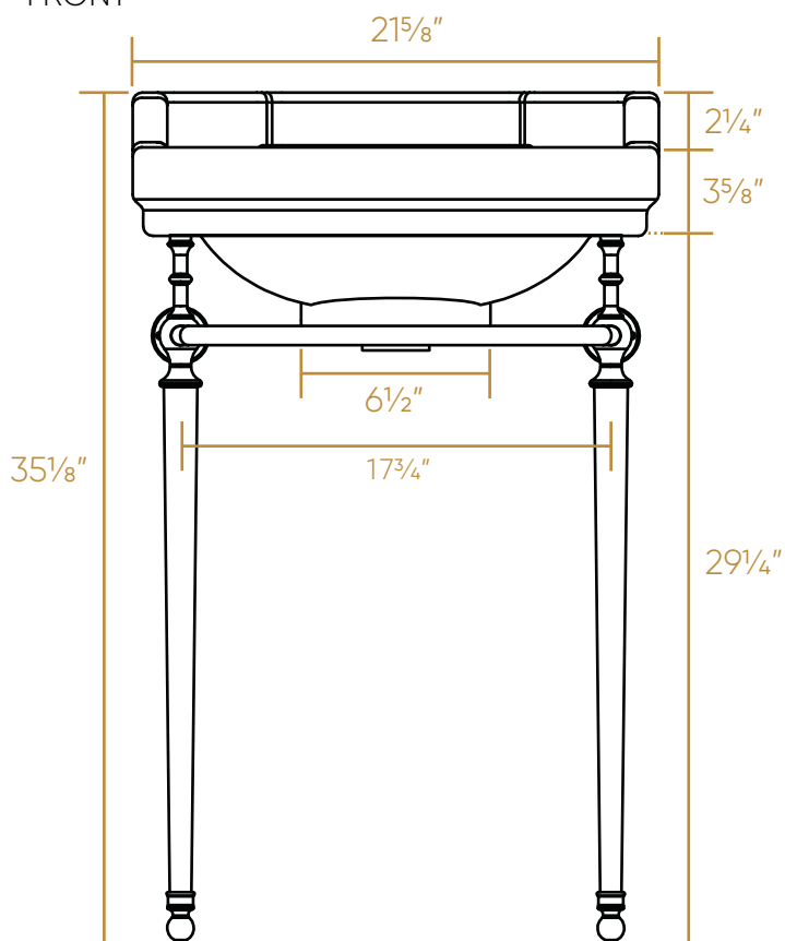
FRONT
