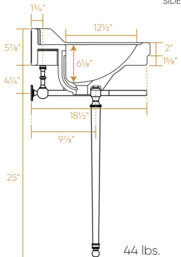
SIDE
